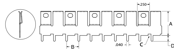
FIGURE 3 .25" Pin Spacing
